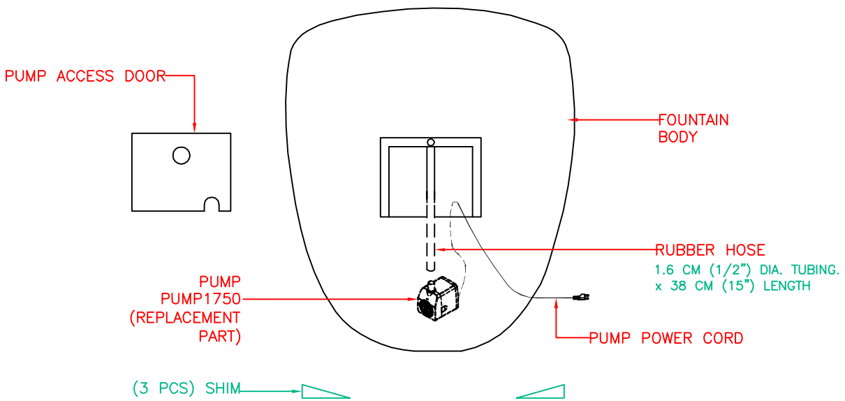
BACK VIEW:
